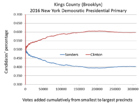
Fig. 15 — 2016 New York Democratic presidential primary Richmond and Kings County, both in New York City, show irregular CVT graphs graphs by Phil Evans
