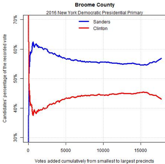
Fig. 22 — 2016 New York Democratic presidential primary, Broome County The CVT graph shows Sanders with an unusual gain in votes in the largest counties A screenshot shows 112.8% reporting, followed by both candidates experiencing a loss of votes graph by Anselmo Sampietro & screenshot courtesy of Aimee Rox Coleman
