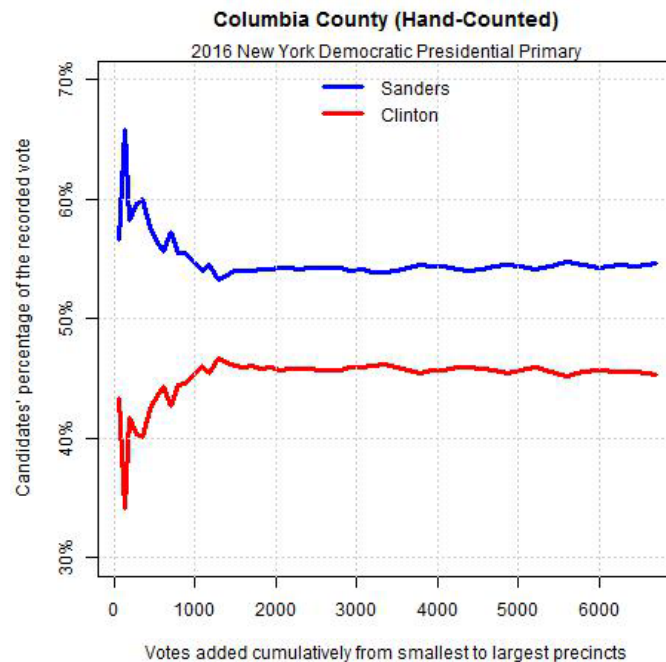
Fig. 17 — 2016 New York Democratic presidential primary, Columbia County This hand-counted county follows the expected statistical pattern Graph by Anselmo Sampietro
